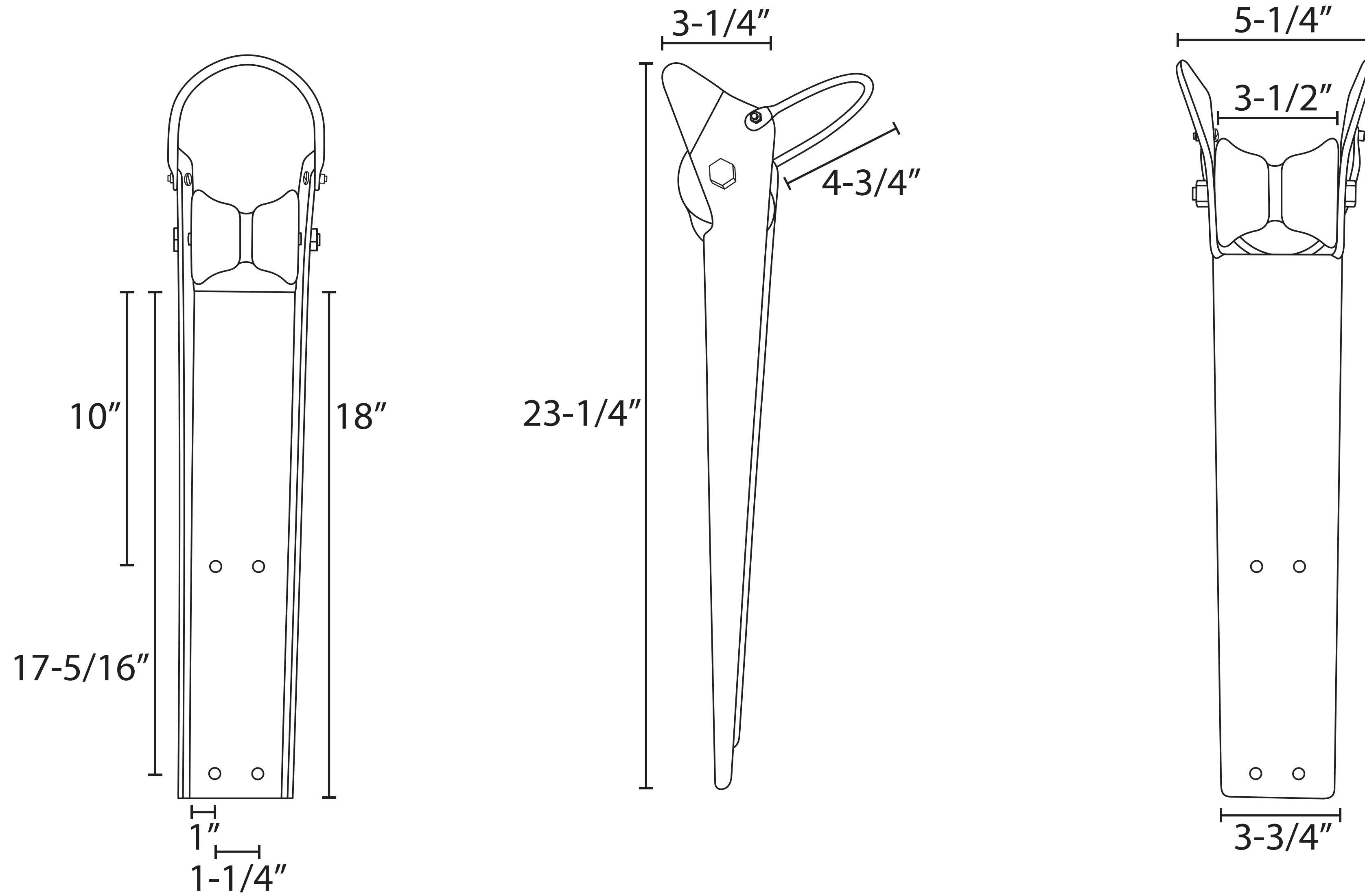
UBR-L Norestar Universal Bow Roller - Large
